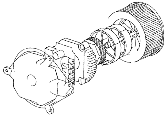
EATC BLOWER MOTOR
