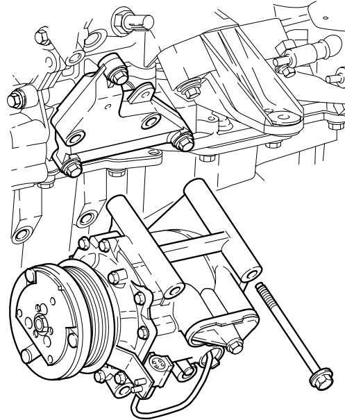
SCROLL-TYPE COMPRESSOR
