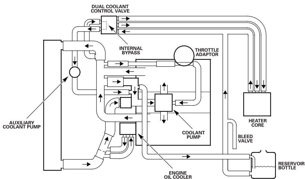
HEATING / COOLING SYSTEM: V8
