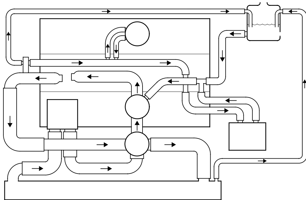
HEATING / COOLING SYSTEM COMPONENTS
