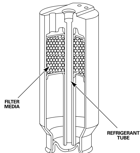
ACCUMULATOR/DRIER
