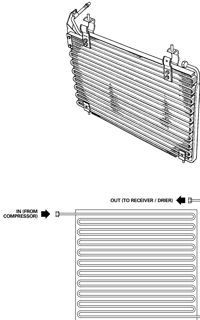
SINGLE PATH CONDENSER
