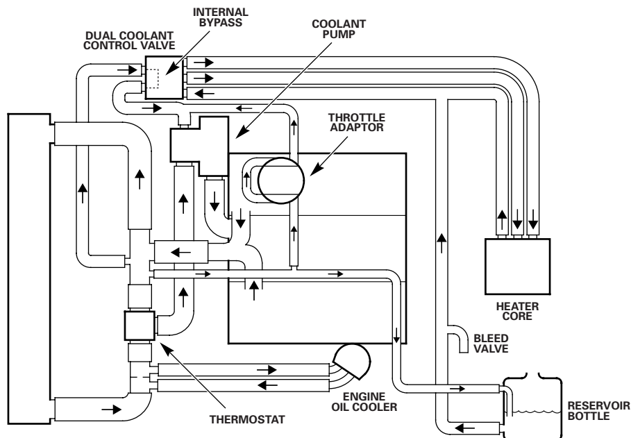
HEATING / COOLING SYSTEM: V6
