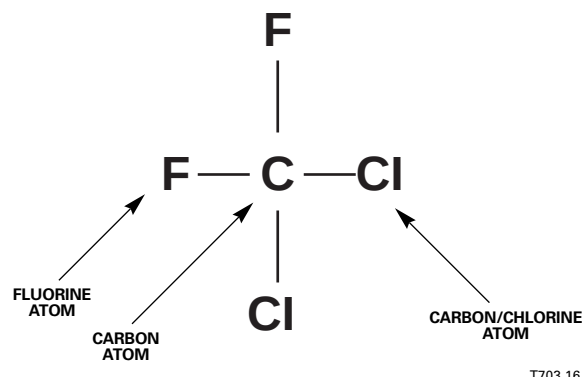
R-12 ATOM STRUCTURE
