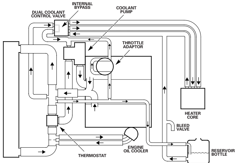
HEATING SYSTEM COMPONENTS (S-TYPE V6 SHOWN)
