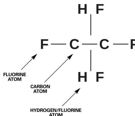
R-134A ATOM STRUCTURE
