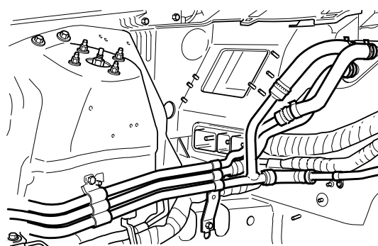
HEATER HOSES
